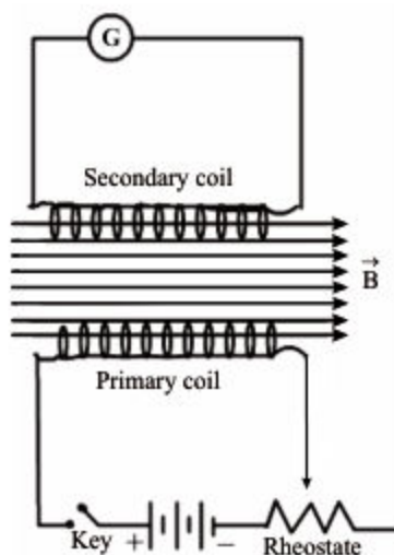
Fig: 16.17 Mutual induction
