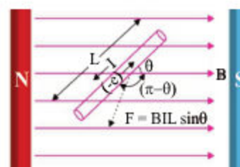
Fig: 16.9 Current carrying conductor in magnetic field
