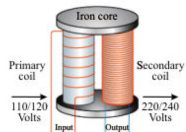
Fig: 16.18 (a) Step up transformer
