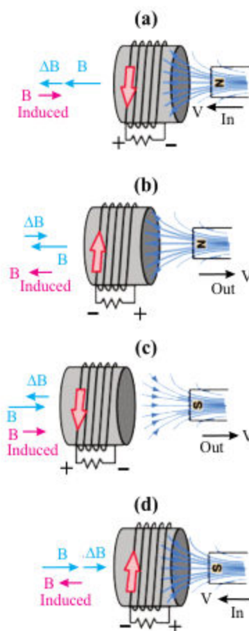
Fig: 16.15 Magnetic field induced by magnetic current
