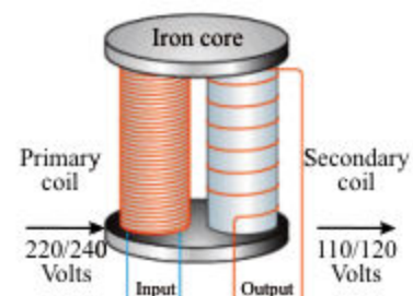
Fig: 16.18 (b) Step down transformer
